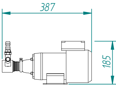
FEED PUMP 12/24V DC
